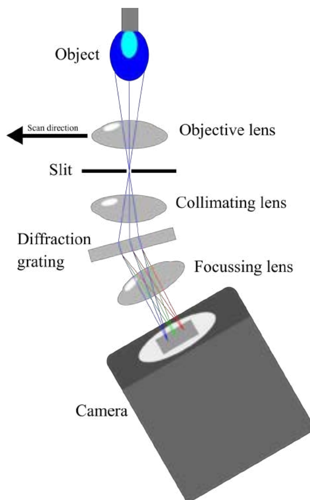
Above: Figure shows the NIR hyperspectral imaging system under development.
