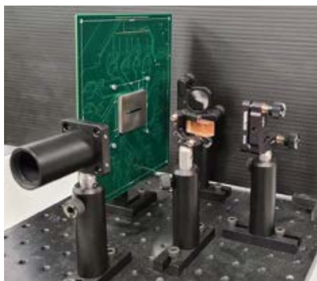
Above: Ultra low cost mid-wave infrared spectrometer.
