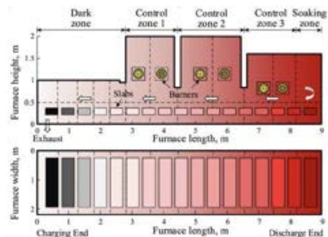
Above: Illustration of a real-world furnace, and its subdivision as different zones.
